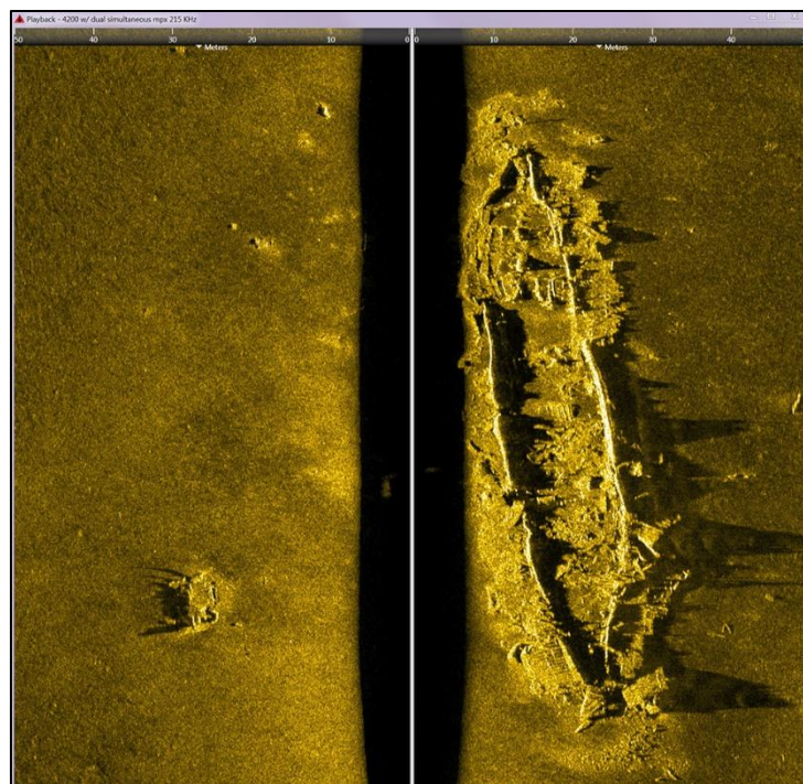
Figure 8 SSS Image of Shipwreck on Seabed and Nadir Gap
