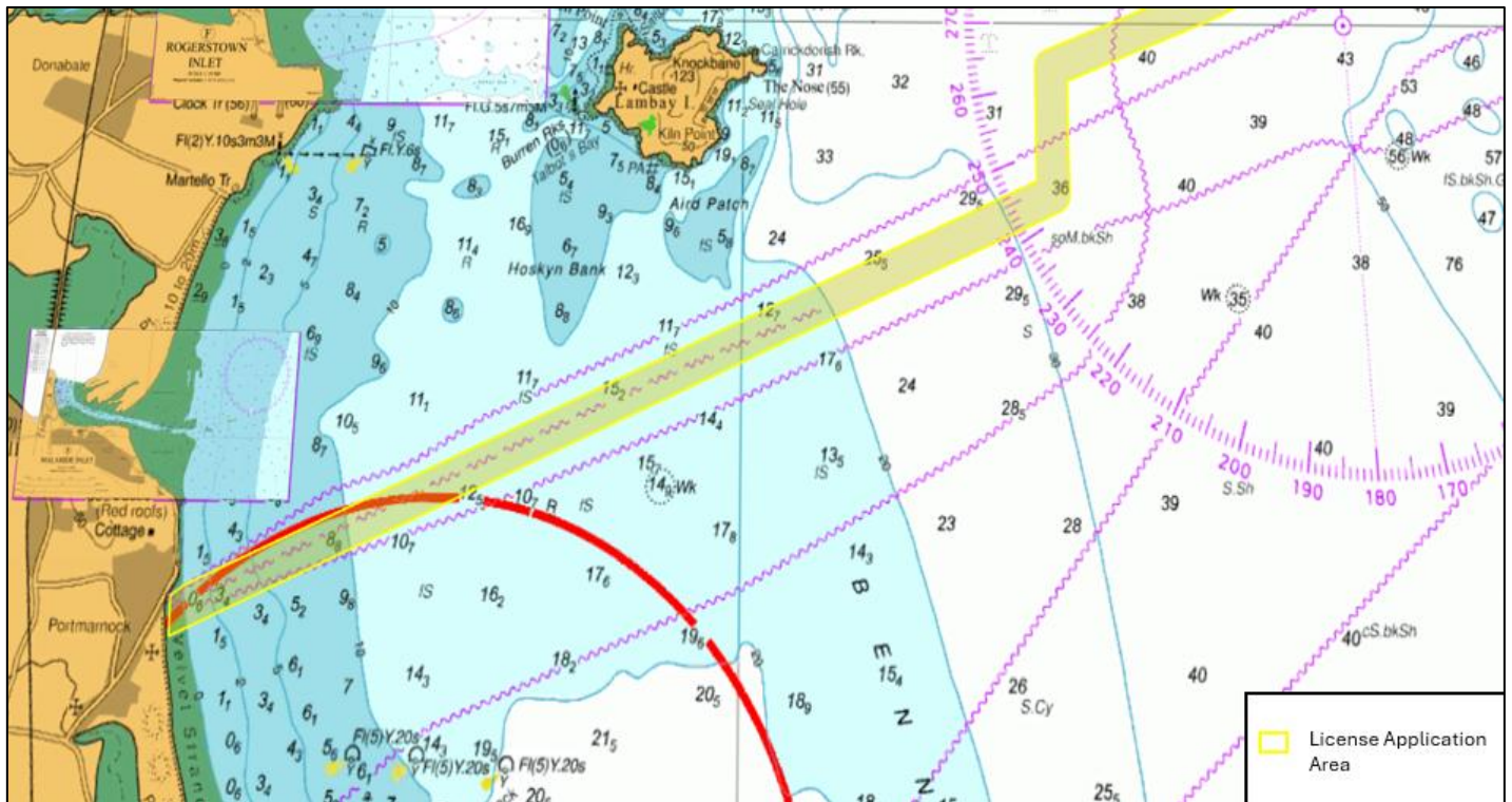
Figure 5 Inshore Survey Sections and Landfalls.
