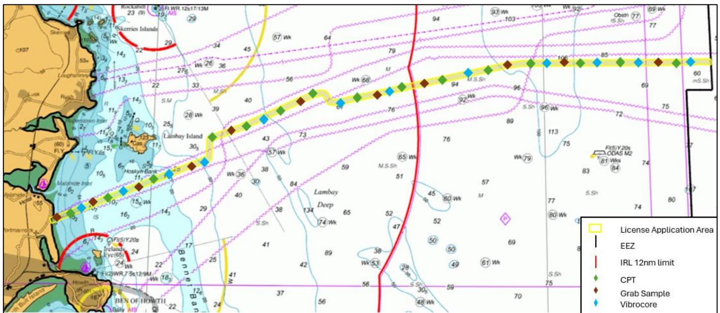
Figure 6 Indicative CPT and Vibrocore Locations
