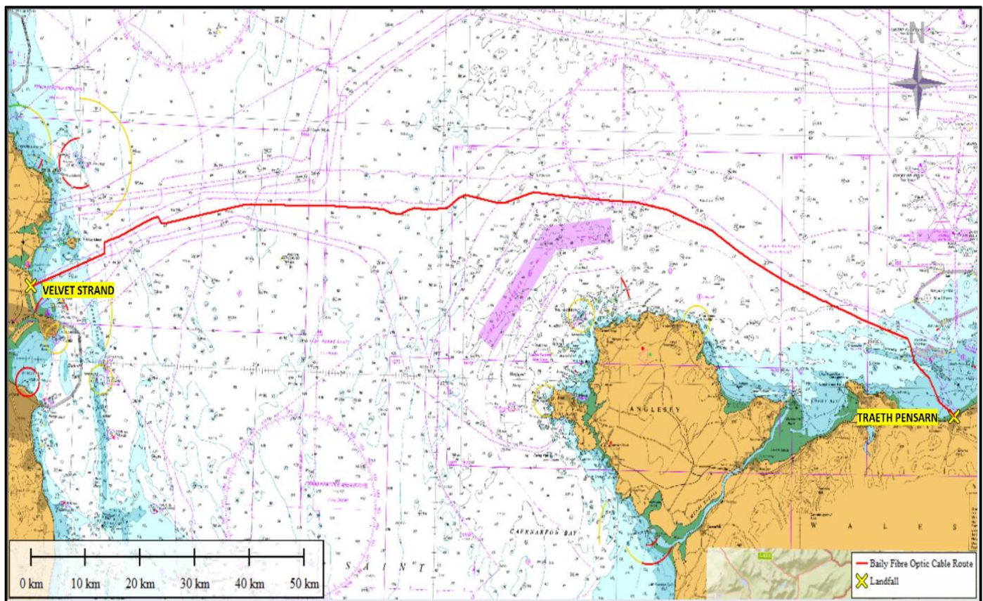
Figure 1 Proposed Baily Telecoms Cable System
