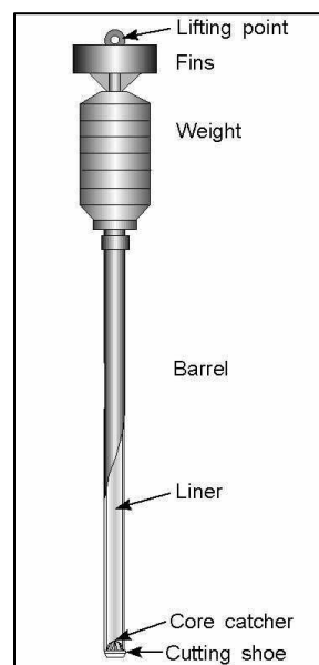
Figure 14 Gravity Corer schematic.
