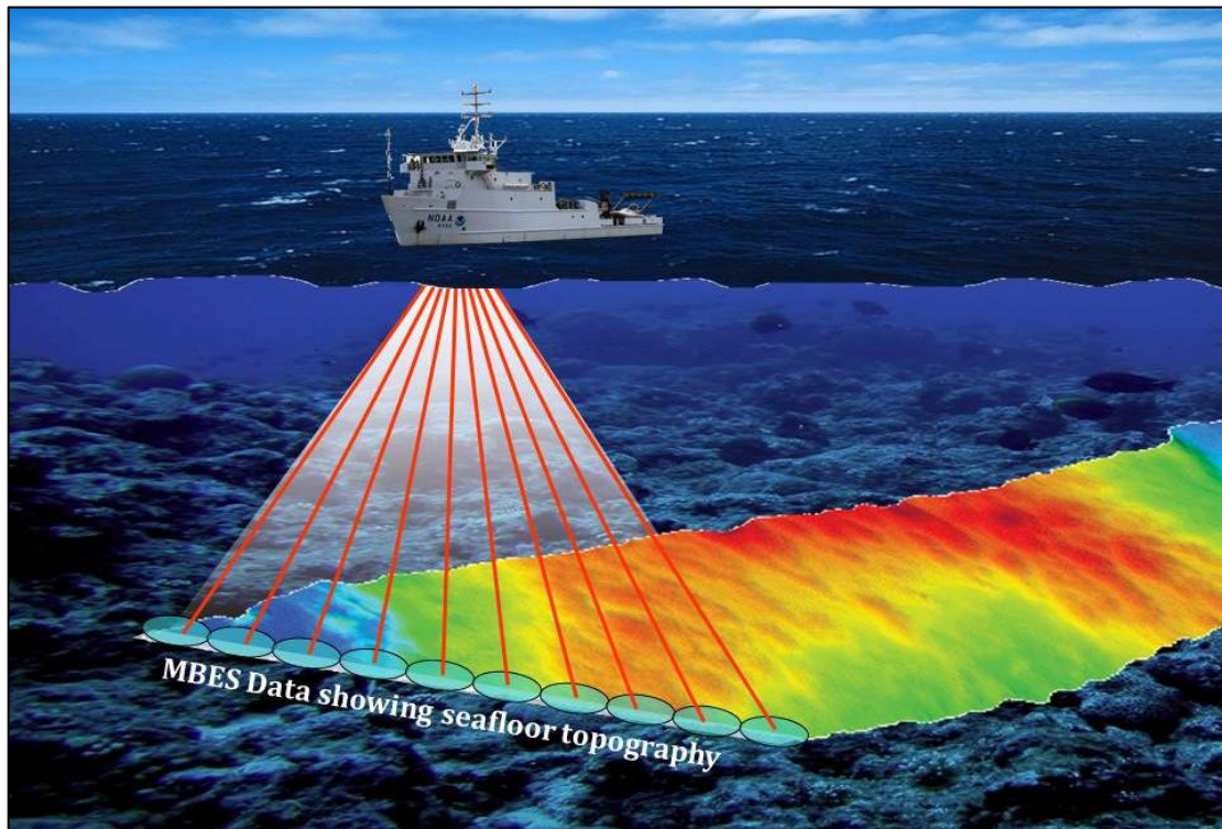
Figure 7 Graphic of MBES Survey in Operation
