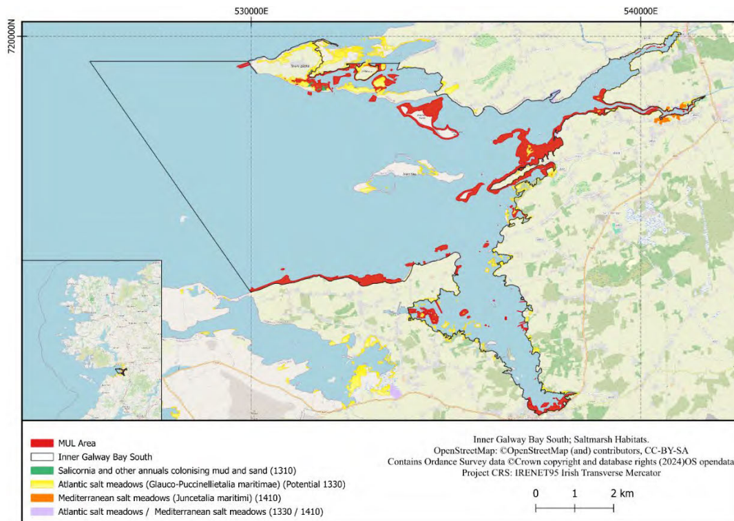
Figure 7 - Saltmarsh Habitats
