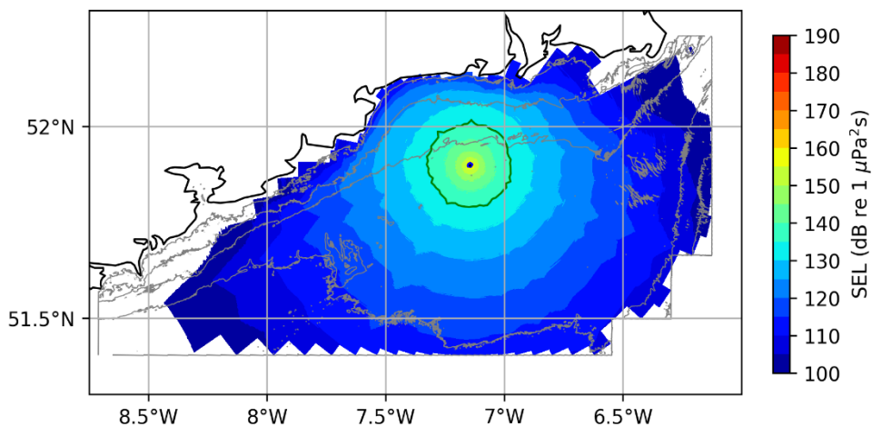
Figure 4.9 Unweighted SEL related to operation of the mini airgun in the project area, showing ranges of PTS_{cum} , TTS_{cum} and the behavioural response effects on the Atlantic herring (blue indicates TTS_{cum} , black: PTS_{cum} and green: behavioural response; cumulation is performed for 1 h)
