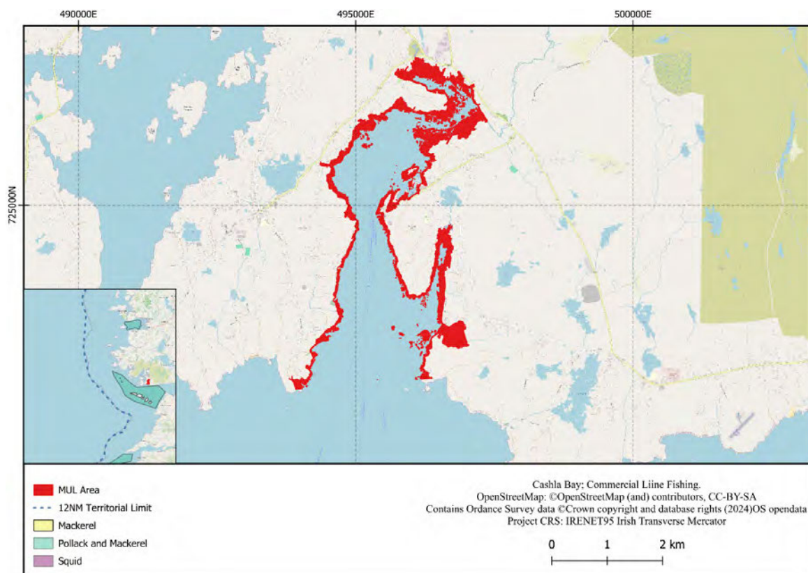
Figure 18 - Commercial fisheries in the vicinity of the MUL area (line fishing)
