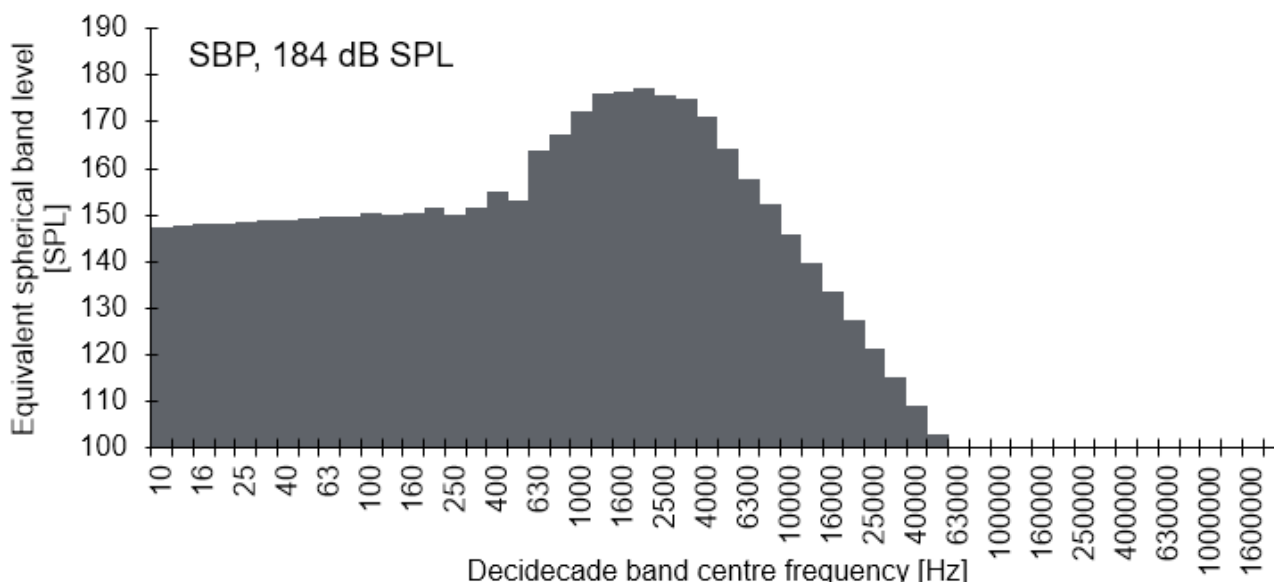
Figure 4-9. Chirper/Pinger type SBP band levels.
