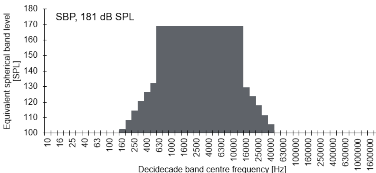
Figure 4-8. Chirper/Pinger type SBP band levels.
