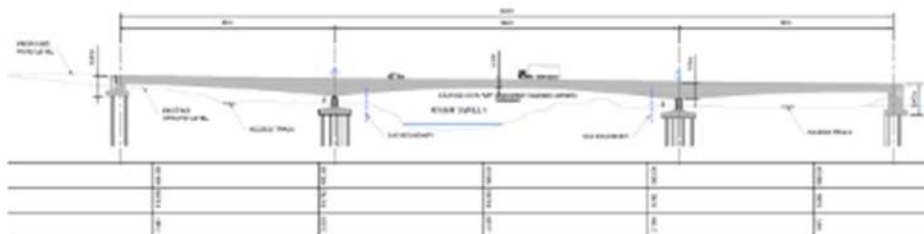
Figure 2.2 River Swilly Crossing – Longitudinal Section
