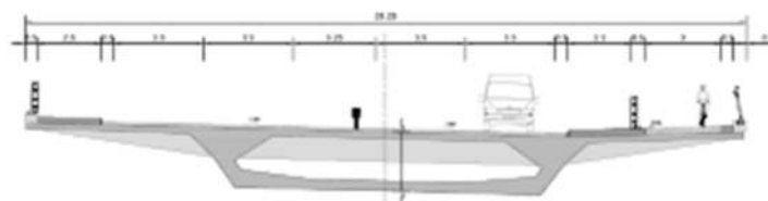
Figure 2.2 River Swilly Crossing – Cross Section at Mid Span
