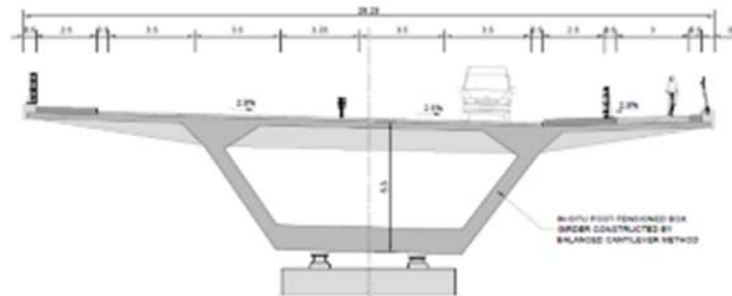
Figure 2.3 River Swilly Crossing – Cross Section at Pier Support
