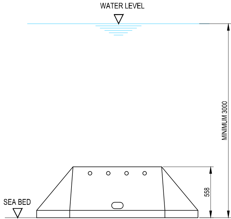
SIDE ELEVATION
