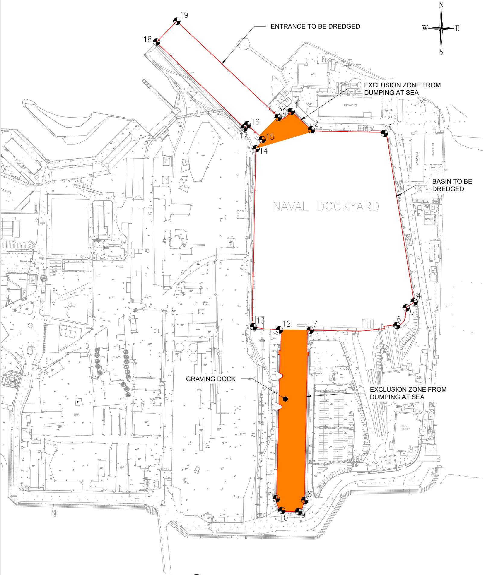
PROPOSED DREDGING ARRANGEMENT Scale 1:2,500
