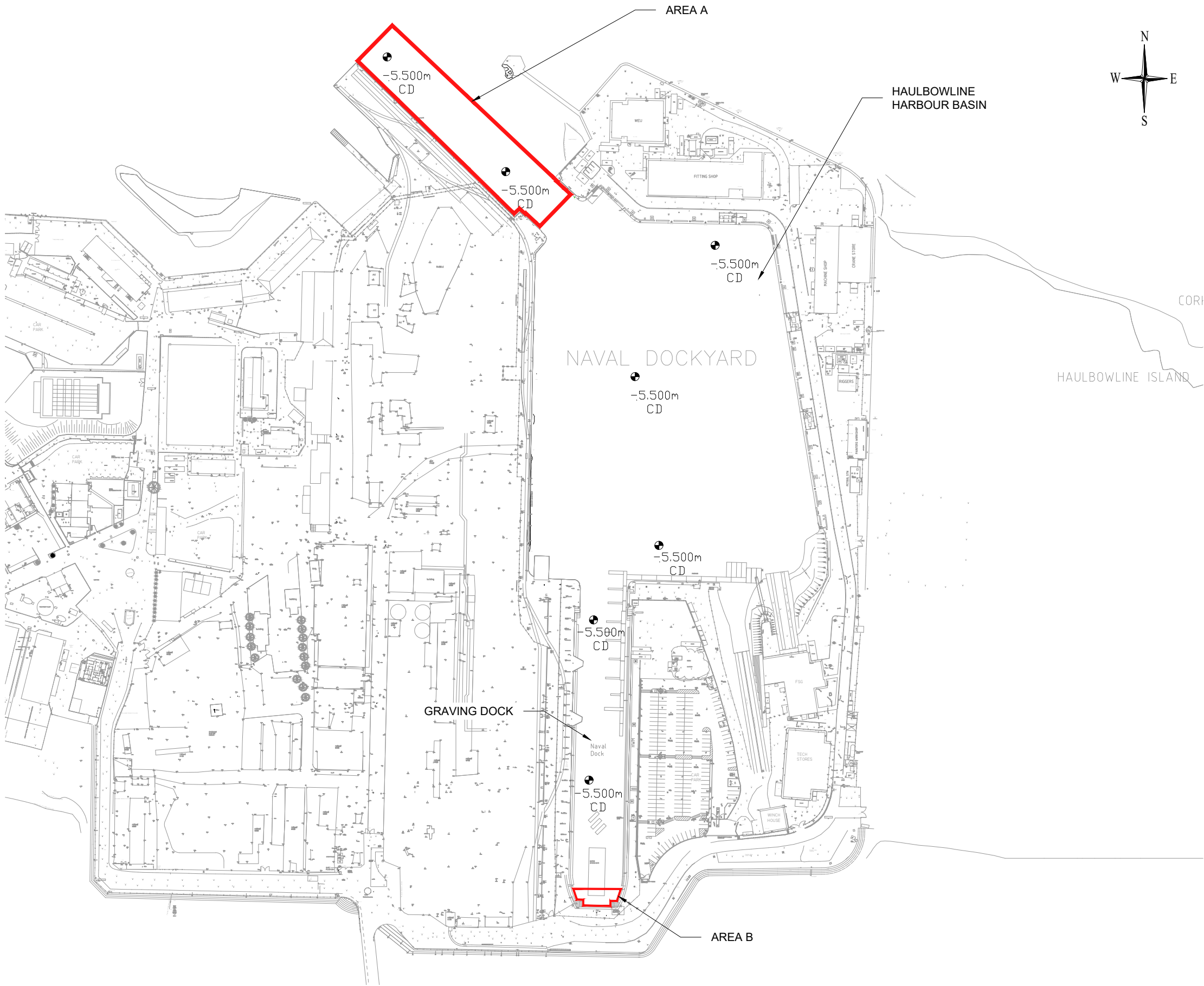
— POST DREDGING ARRANGEMENT — Scale 1:2,500
